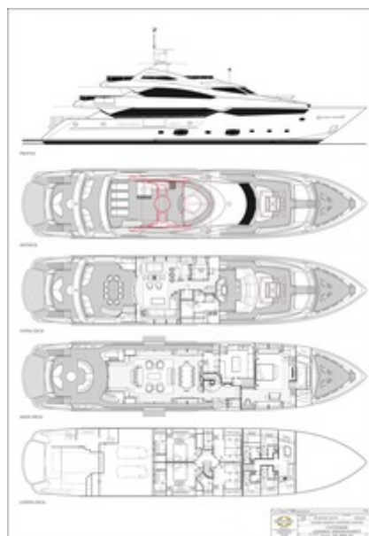
General layout
